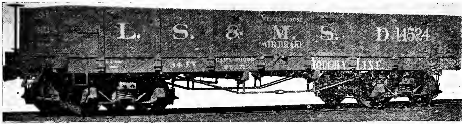
Fig. 22. GONDOLA CAR, SINGLE DROP-BOTTOM, FOR COAL AND LUMBER. LAKE SHORE & MICHIGAN SOUTHERN RAILWAY. Length, 34 ft. Capacity, 60,000 lbs. Weight, 27,150 lbs. Equipped with Air Brakes and Rigid Diamond Trucks.
